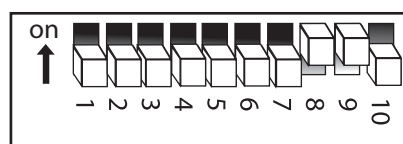
Dipswitches 1-8 (programmes)
